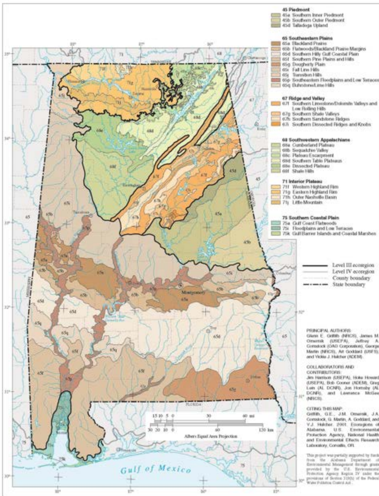
Figure 1-2 Alabama's Level III and IV Ecoregions
