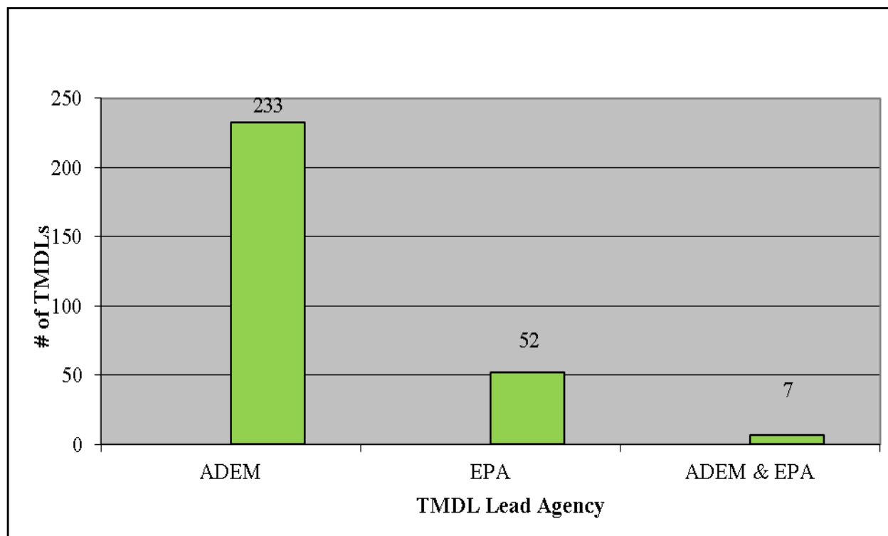
Figure 9-1 Alabama's Approved TMDLs in Alabama
